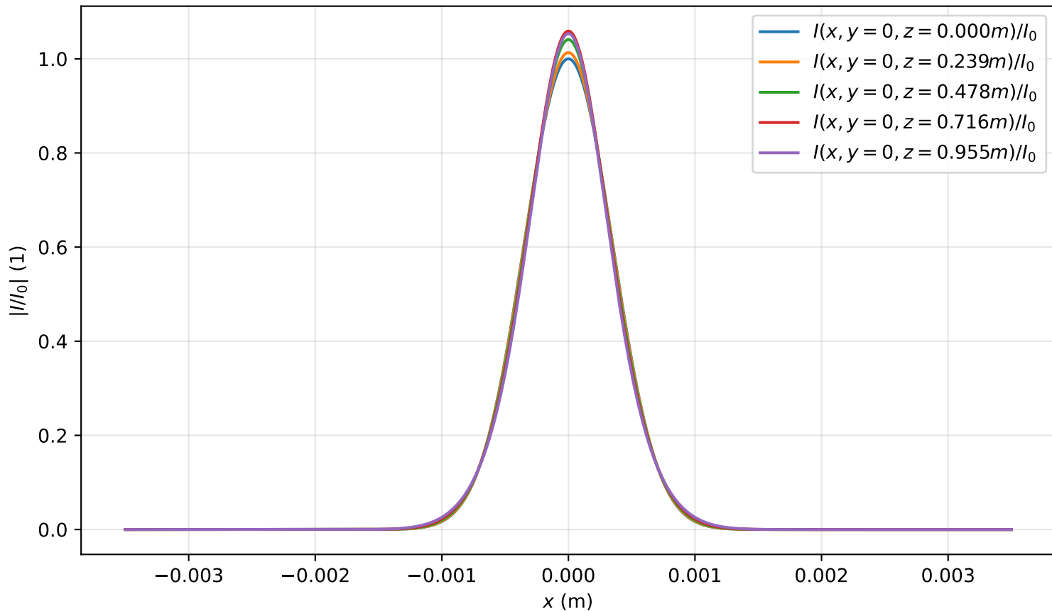
Intensity profile I(x, y = 0, z)/I_0 , P_{in}=6.5P_{cr} , artificial time
